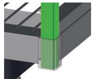
ORDER PICKING CONTAINER Basic model with accessories, bolted design Dimensions (mm): W 600 x D 600 x H 1635
