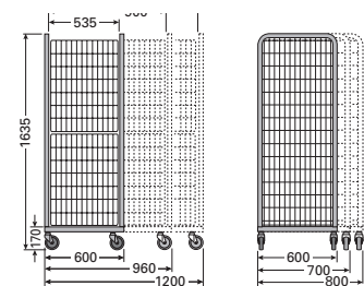
Container with height of 1635 mm, dimensions in mm
