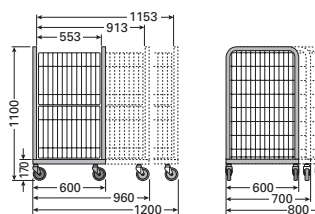
Container with height of 1100 mm, dimensions in mm
