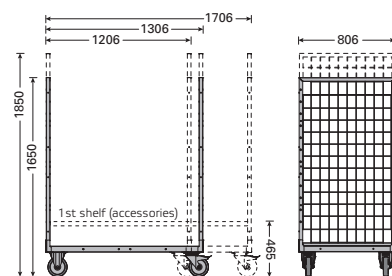
KT4 with depth of 806 mm, dimensions in mm
