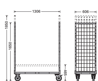
KT4 with depth of 606 mm, dimensions in mm
